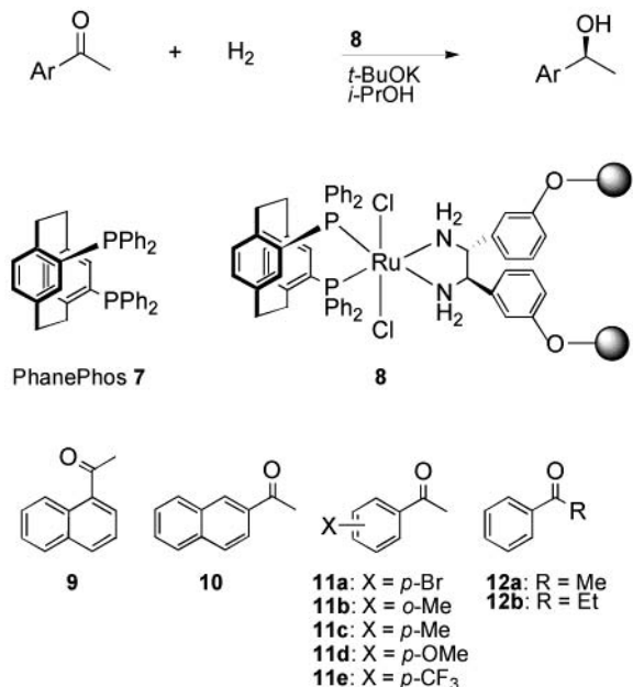
Scheme 2. Asymmetric Hydrogenation of Ketones with 8
